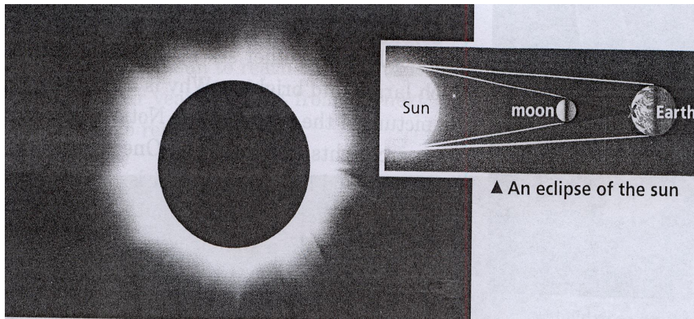
Gambar 6.9 Korona
