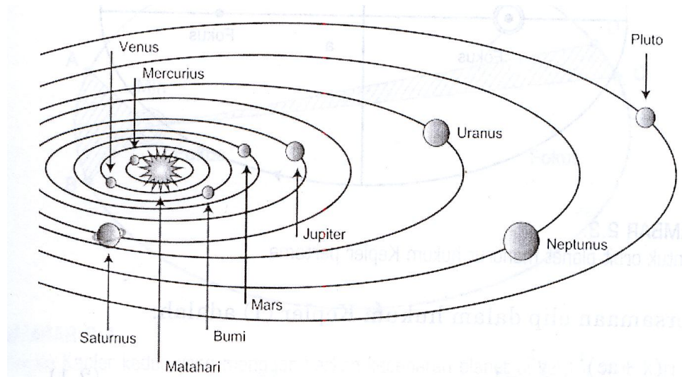
Gambar 6.3 Sistem Tata Surya Heliosentris
