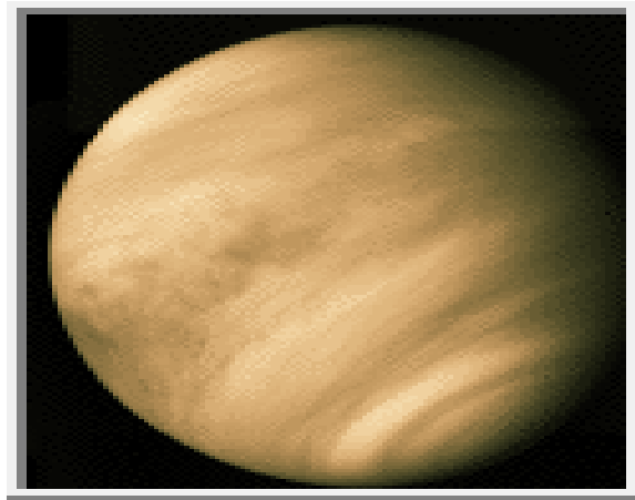
Gambar 6.11 Planet Venus
