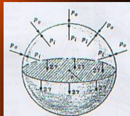
FIGURE 9.8 Forces on one hemisphere of a bubble produced by the air pressure inside and outside the bubble and by the surface tension exerted by the other hemisphere.
