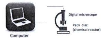
Figure 2. Schematic arrangement of the solid-liquid chemical reaction observation kits
