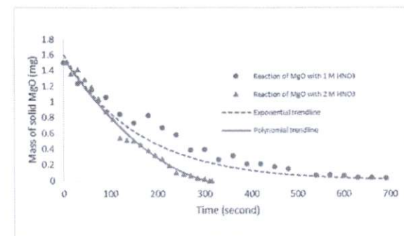
Figure 6. Plot of MgO mass against reaction time observed using a microscope and processed using the application with different concentration of HNO 3 .
