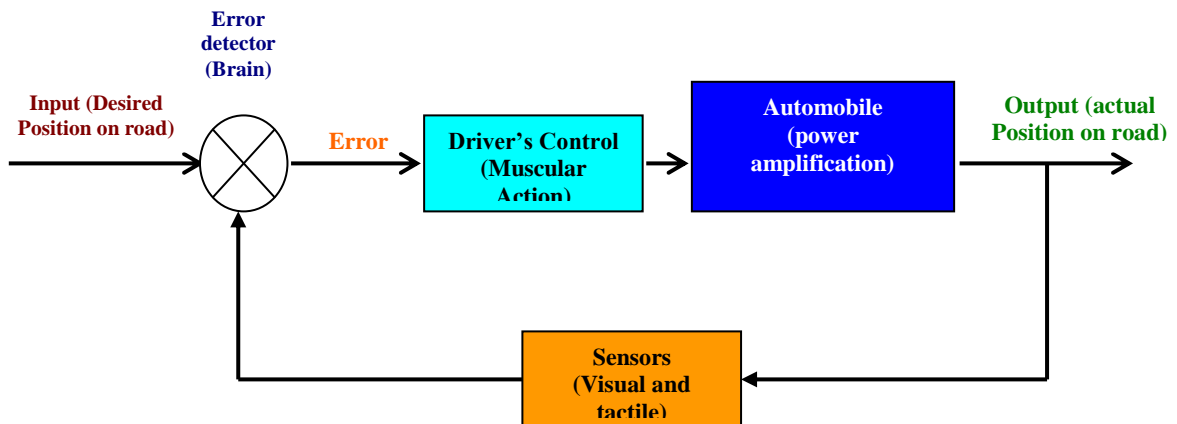
Fig. 1. Steering of an automobile: a feedback control system involving human capability.
