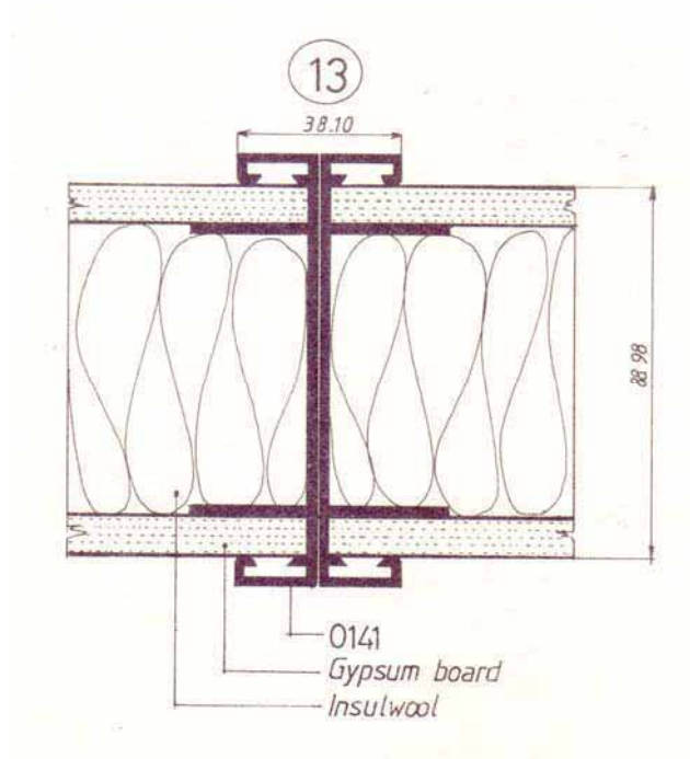
Gambar.21 Detail 13 Partition
