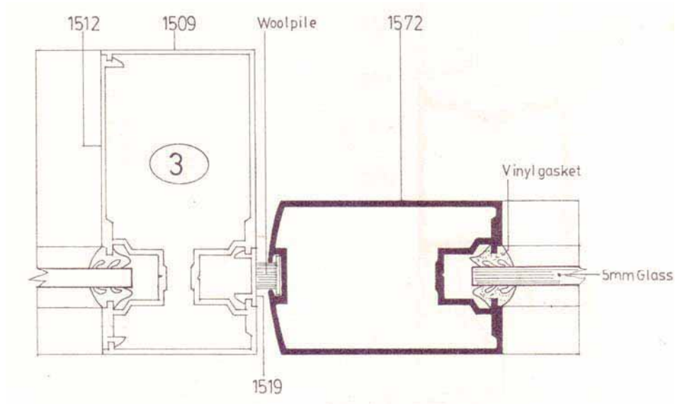
Gambar 5 Detail 3 Kosen Pintu (Swing Door)
