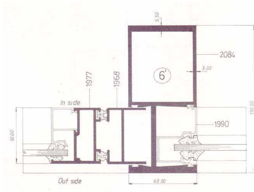
Gambar.13 Detail 6' Curtain Wall
