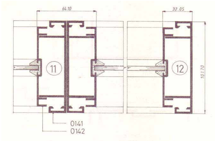
Gambar.20 Detail 11-12 Partition
