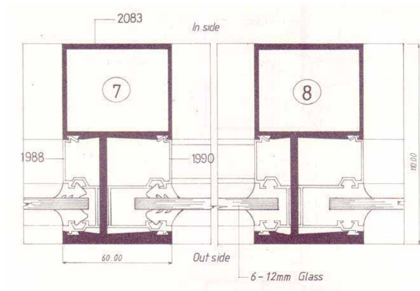
Gambar.14 Detail 7-8 Curtain Wall
