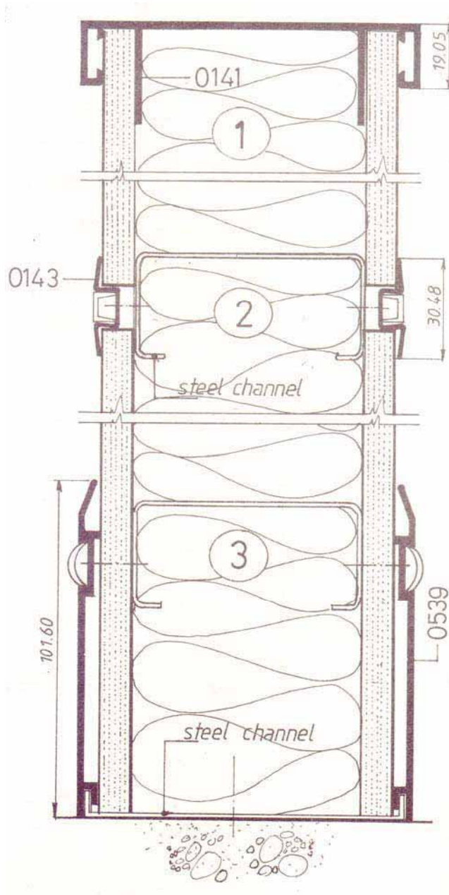
Gambar.16 Detail 1-3 Partition
