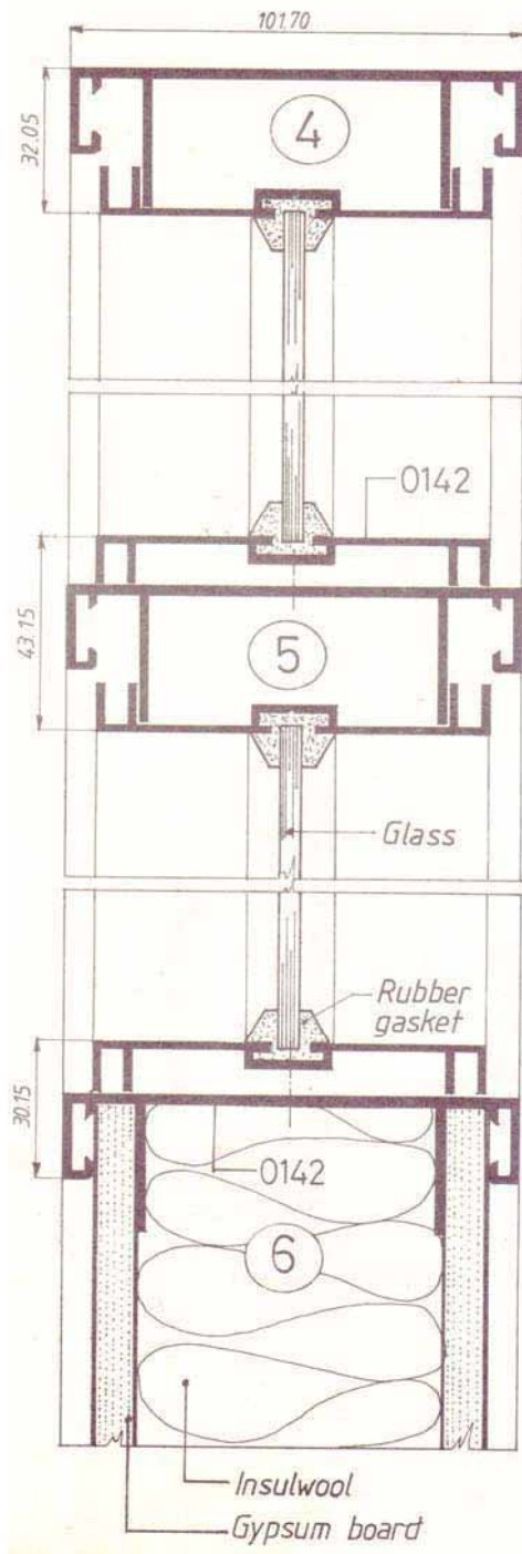
Gambar.17 Detail 4-6 Partition
