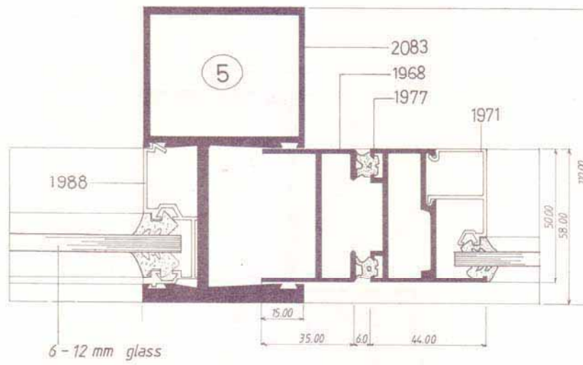
Gambar.11 Detail 5 Curtain Wall
