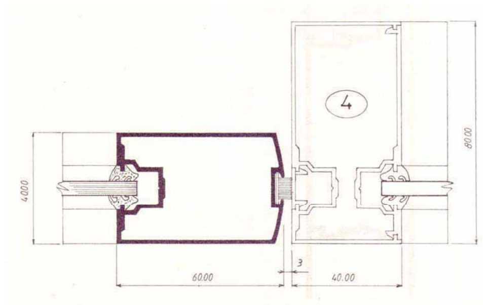
Gambar 6 Detail 4 Kosen Pintu (Swing Door)
