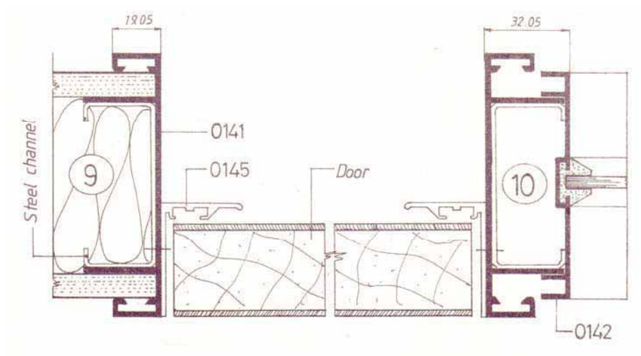
Gambar.19 Detail 9-10 Partition
