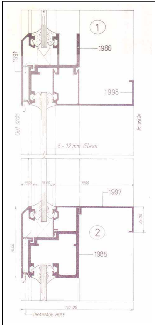
Gambar 9 Detail 1-2 Curtain Wall
