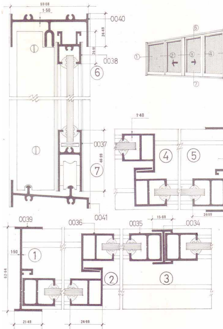
Gambar 7 Jendela Sorong (Sliding Window)
