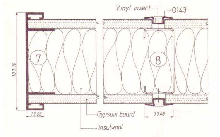
Gambar.18 Detail 7-8 Partition
