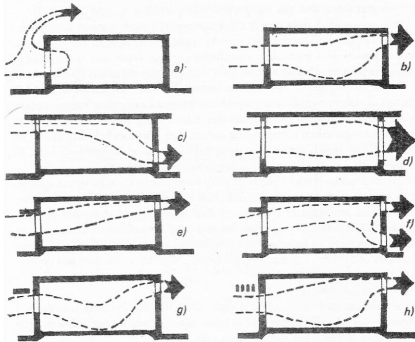
Ventilasi silang (horizontal) hasil penelitian dari Texas Engineering Experiment Station
