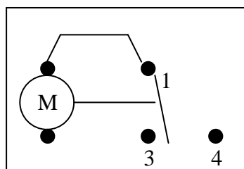
Gambar 8. Timer
