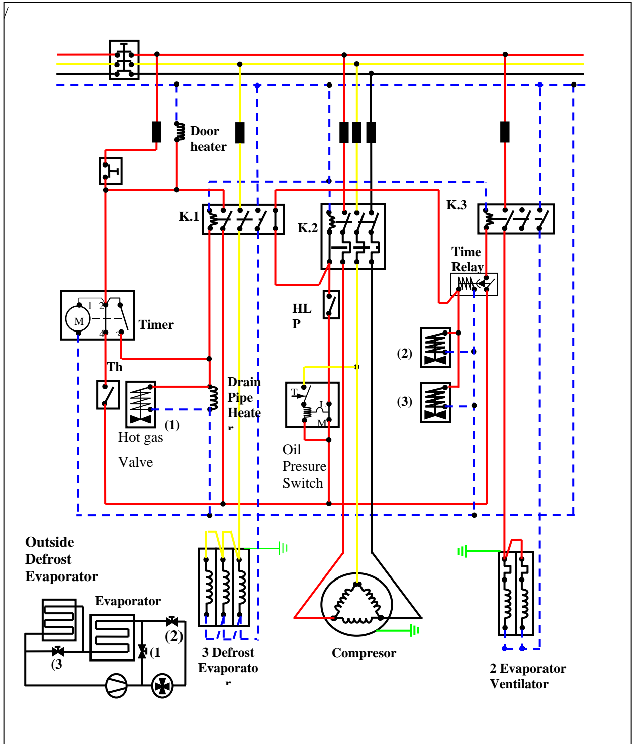
RANGKAIAN SISTEM REFRIGERATION SYSTEM WITH HOT GAS DEFROST AND VENTILATOR START DELAY
