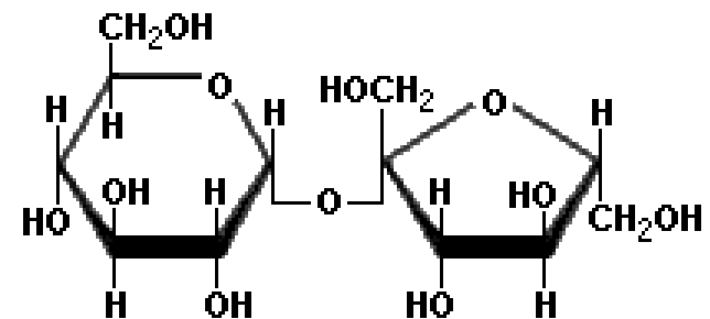
Sucrose
