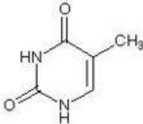
Timin
