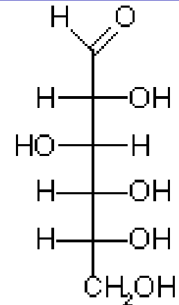
D-Glucose
