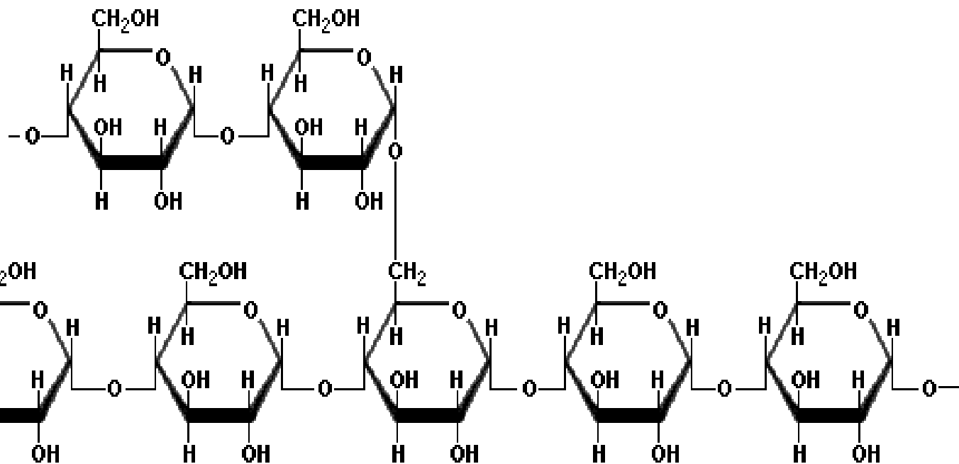
Amylopectin
