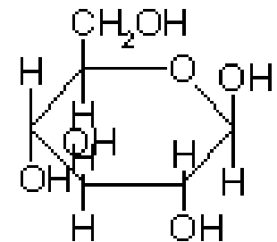
D-Glucose
