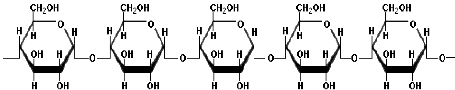
Amylose
